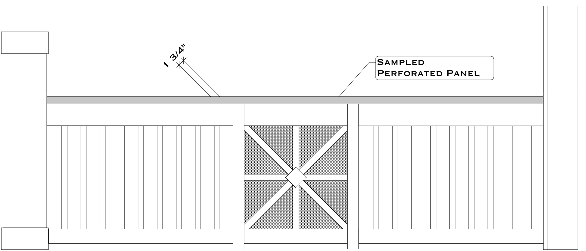
DECK VIEW SCALE: 3/4" = 1'-0"
