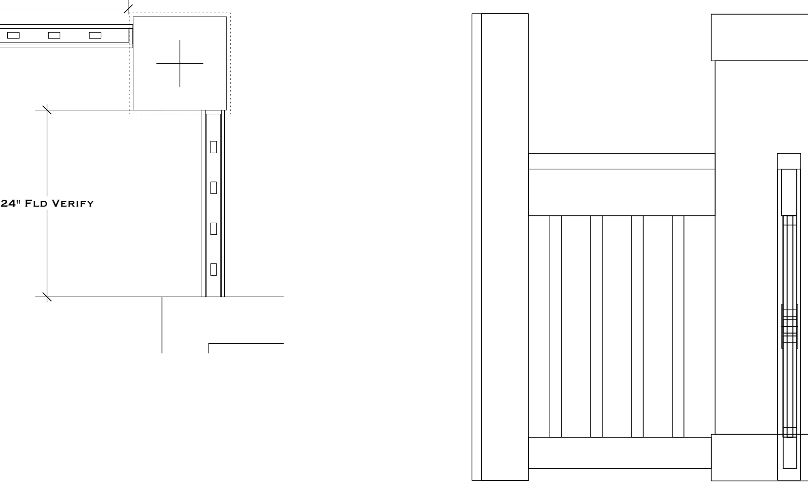
SIDE VIEW STD BALCONY SCALE: 1" = 1'-0"
