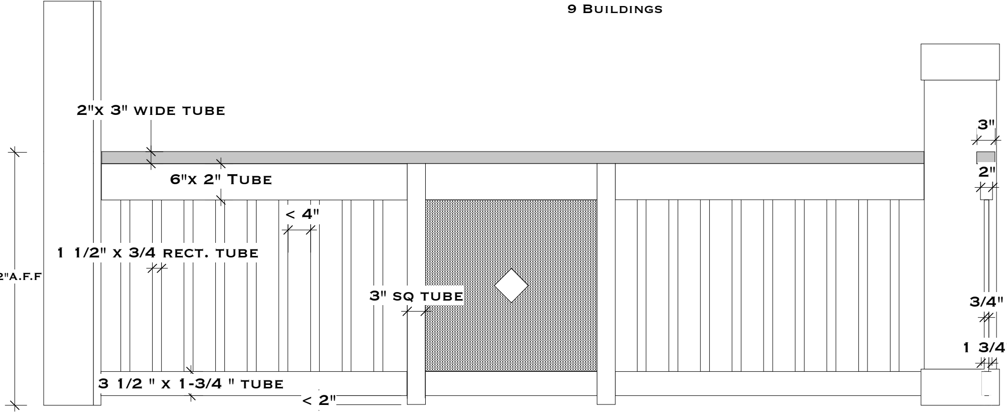
DECK VIEW SCALE: 3/4" = 1'-0"
